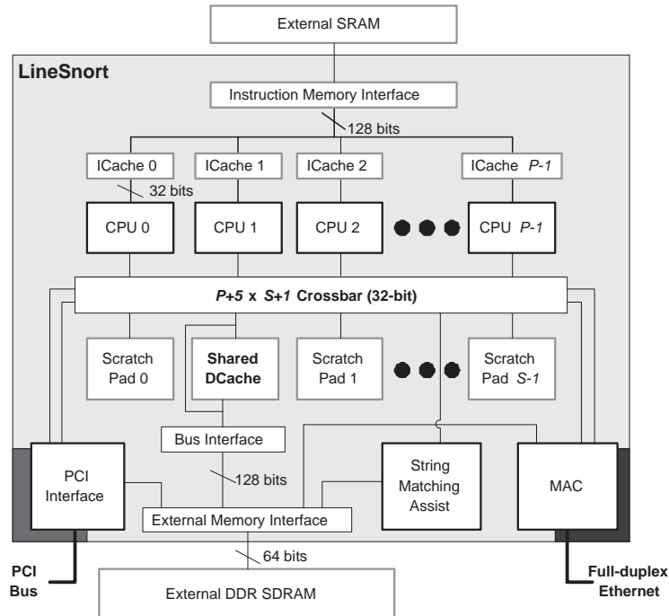
Figure 2. Block diagram of proposed Ethernet controller architecture
